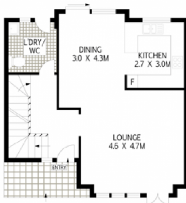
GROUND LEVEL
