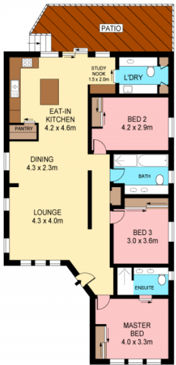
GROUND FLOOR
