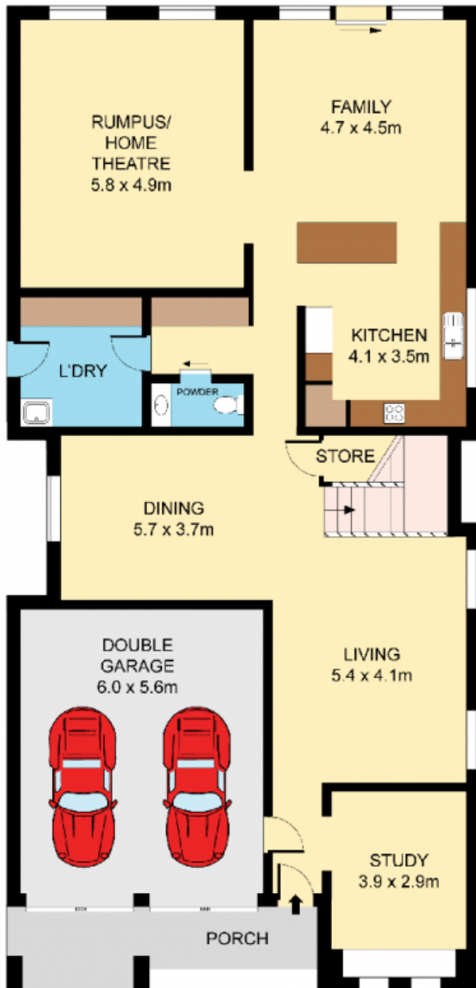
GROUND FLOOR
