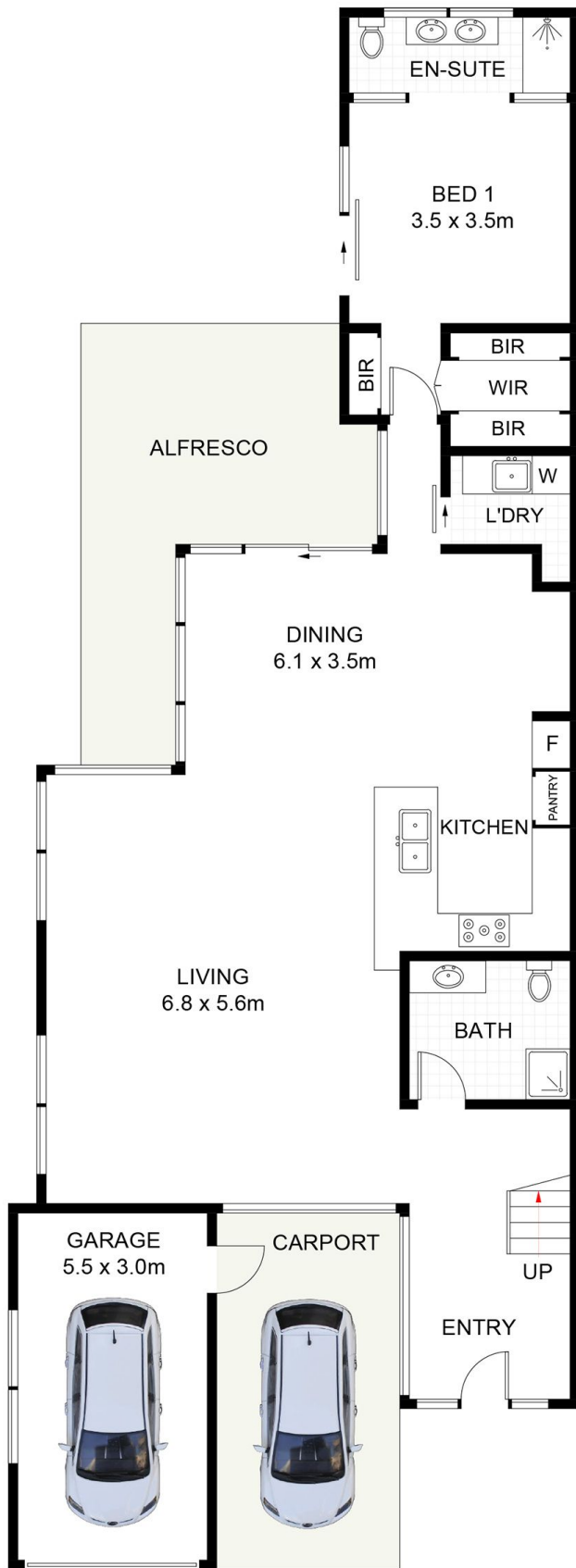
GROUND FLOOR
