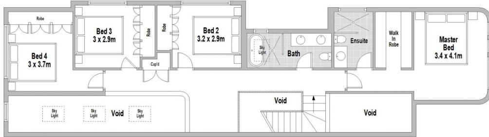
FIRST FLOOR
